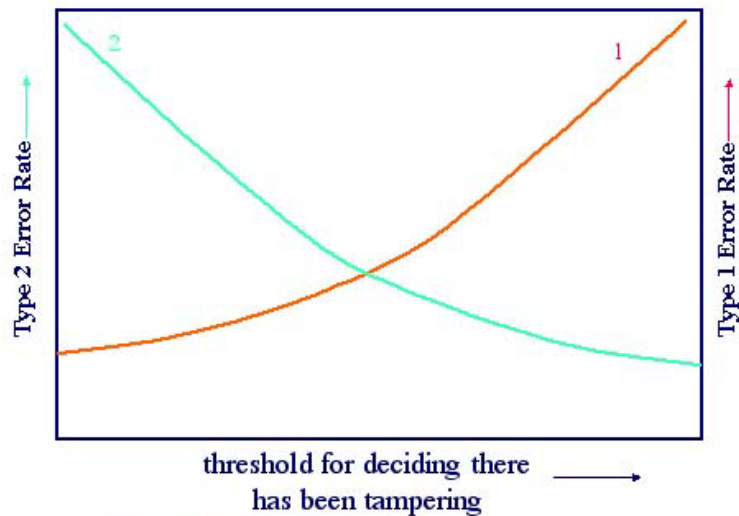
Figure 1 - Low rates of Type 2 errors typically come at the cost of relatively high rates for Type 1 errors, and vice versa
